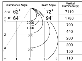
■ Direct Horizontal Illuminance SD346-42B8027
