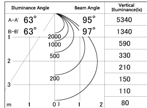
■ Direct Horizontal Illuminance SD347-36B8527
