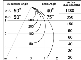
■ Direct Horizontal Illuminance DD054-08MB9027-DM
