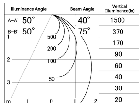
■ Direct Horizontal Illuminance DD054-08MB9040-DM
