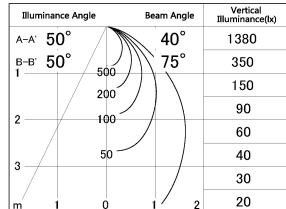
■ Direct Horizontal Illuminance DD054-08MW9027
