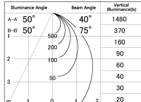
■ Direct Horizontal Illuminance DD054-08MW9035
