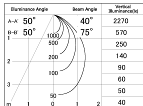
■ Direct Horizontal Illuminance DD054-13MB9027
