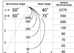
■ Direct Horizontal Illuminance DD054-13MB9030
