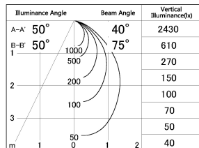
■ Direct Horizontal Illuminance DD054-13MB9035-DM
