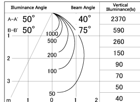
■ Direct Horizontal Illuminance DD054-13MW9030
