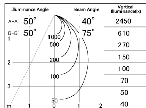
■ Direct Horizontal Illuminance DD054-13MW9040-DM
