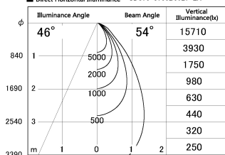
■ Direct Horizontal Illuminance SD376-3755B9027-LX
