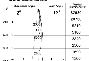
■ Direct Horizontal Illuminance SD376-2015B9027-LX
