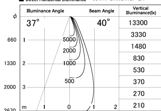
■ Direct Horizontal Illuminance SD376-2035B9027-LX
