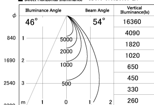
■ Direct Horizontal Illuminance SD376-3755B9030-LX
