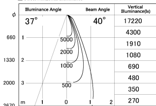
■ Direct Horizontal Illuminance SD376-2535B9030-LX
