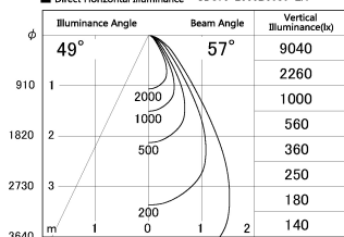
■ Direct Horizontal Illuminance SD376-2555B9030-LX
