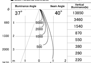
■ Direct Horizontal Illuminance SD376-2035B9030-LX
