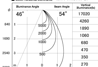
■ Direct Horizontal Illuminance SD376-3755B9035-LX
