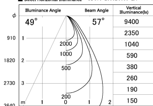
■ Direct Horizontal Illuminance SD376-2555B9035-LX
