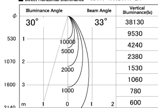
■ Direct Horizontal Illuminance SD376-4035B9040-LX
