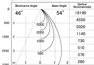
■ Direct Horizontal Illuminance SD376-4055B9040-LX
