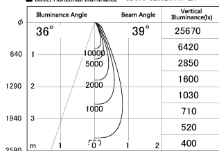
■ Direct Horizontal Illuminance SD376-3235B9040-LX
