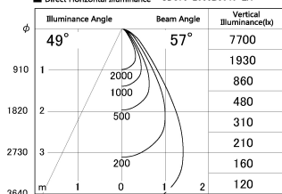
■ Direct Horizontal Illuminance SD376-2055B9040-LX
