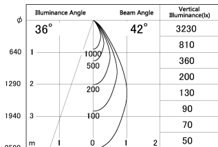
■ Direct Horizontal Illuminance SD287-0650W9030-DMWL
