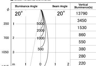
■ Direct Horizontal Illuminance SD287-0625W9035-DMWL
