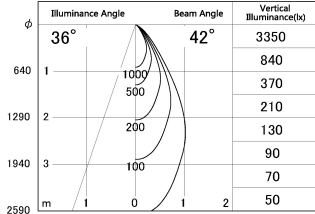
■ Direct Horizontal Illuminance SD287-0650W9035-DMWL
