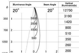
■ Direct Horizontal Illuminance SD287-0625B9027-DMWL
