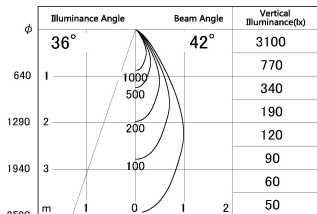
■ Direct Horizontal Illuminance SD287-0650B9027-DMWL
