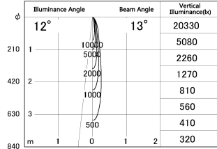
■ Direct Horizontal Illuminance SD287-0615B9030-DMWL
