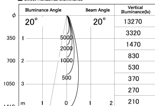
■ Direct Horizontal Illuminance SD287-0625B9030-DMWL
