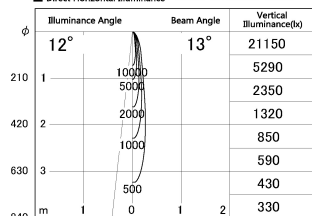
■ Direct Horizontal Illuminance SD287-0615B9035-DMWL
