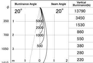
■ Direct Horizontal Illuminance SD287-0625B9035-DMWL
