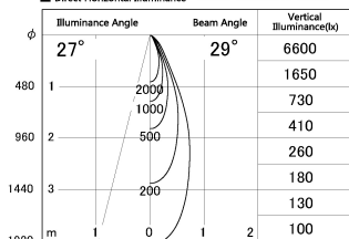
■ Direct Horizontal Illuminance SD287-0635B9040-DMWL
