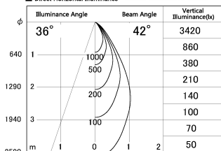
■ Direct Horizontal Illuminance SD287-0650B9040-DMWL
