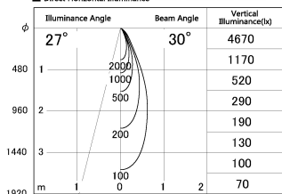
■ Direct Horizontal Illuminance SD287-0635WHC27-DMWL
