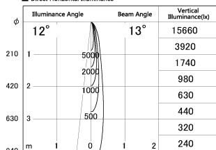
■ Direct Horizontal Illuminance SD287-0615WHC30-DMWL
