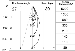
■ Direct Horizontal Illuminance SD287-0635WHC35-DMWL
