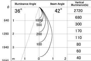
■ Direct Horizontal Illuminance SD287-0650WHC35-DMWL
