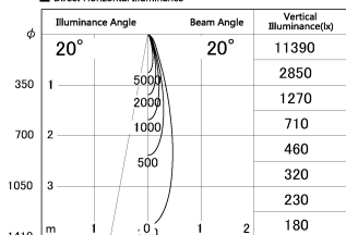
■ Direct Horizontal Illuminance SD287-0625WHC40-DMWL
