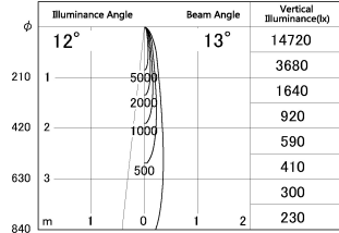
■ Direct Horizontal Illuminance SD287-0615BHC27-DMWL
