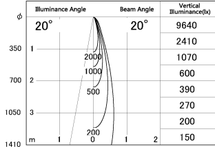
■ Direct Horizontal Illuminance SD287-0625BHC27-DMWL
