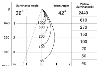
■ Direct Horizontal Illuminance SD287-0650BHC27-DMWL
