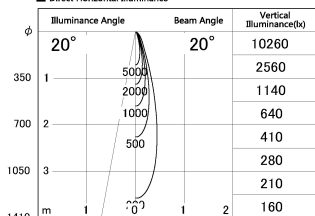
■ Direct Horizontal Illuminance SD287-0625BHC30-DMWL
