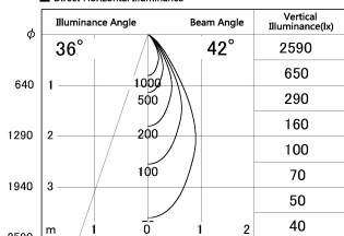
■ Direct Horizontal Illuminance SD287-0650BHC30-DMWL
