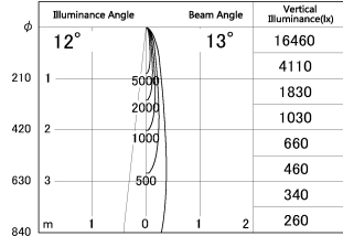
■ Direct Horizontal Illuminance SD287-0615BHC35-DMWL
