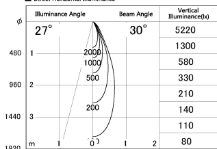
■ Direct Horizontal Illuminance SD287-0635BHC35-DMWL
