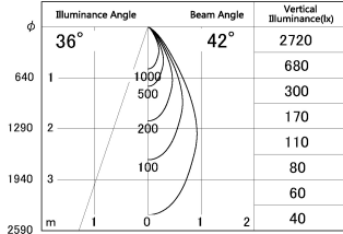
■ Direct Horizontal Illuminance SD287-0650BHC35-DMWL
