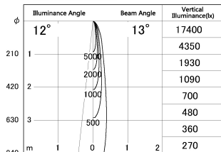
■ Direct Horizontal Illuminance SD287-0615BHC40-DMWL
