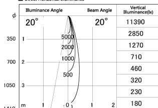
■ Direct Horizontal Illuminance SD287-0625BHC40-DMWL
