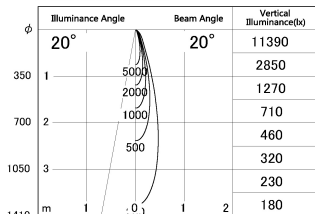
■ Direct Horizontal Illuminance SD287-0625BHC40-DMWL
